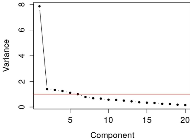
Figure 1 - Screeplot of components. Points above the red line present variances > 1; these are the relevant components.
